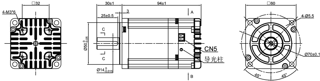
外形图 (DIMENSIONS) unit=mm
